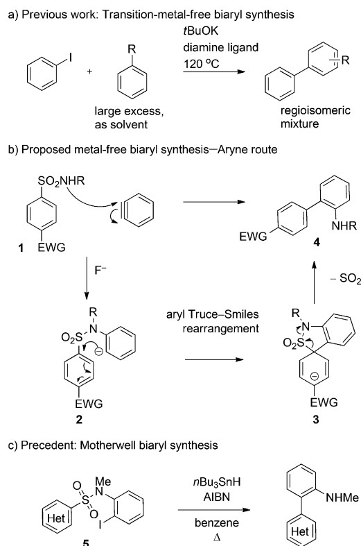
Scheme 1. Proposed aryne addition/Truce–Smiles rearrangement for biaryl synthesis. AIBN = 2,2'-azobis(2-methylpropionitrile), EWG = electron-withdrawing group.
